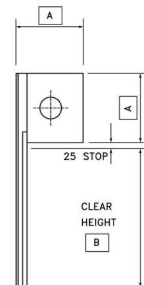
SECTIONAL VIEW
